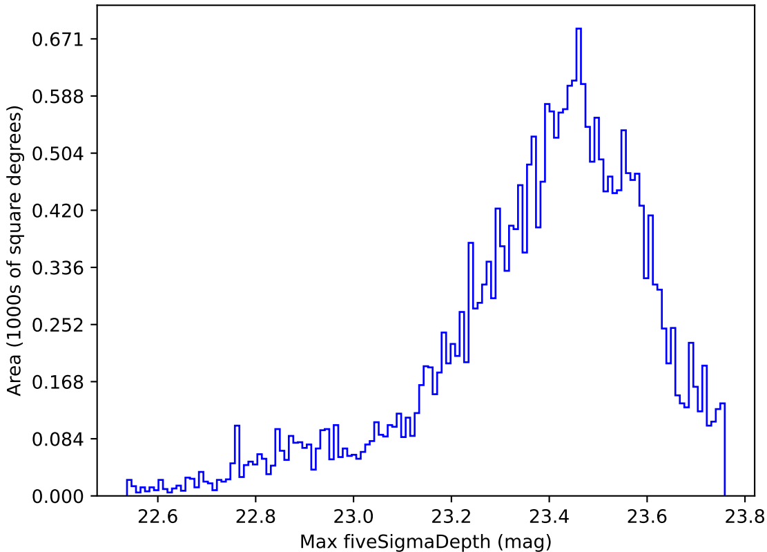
baseline_v3.5_10yrs Yr 1 z band: Max fiveSigmaDepth
