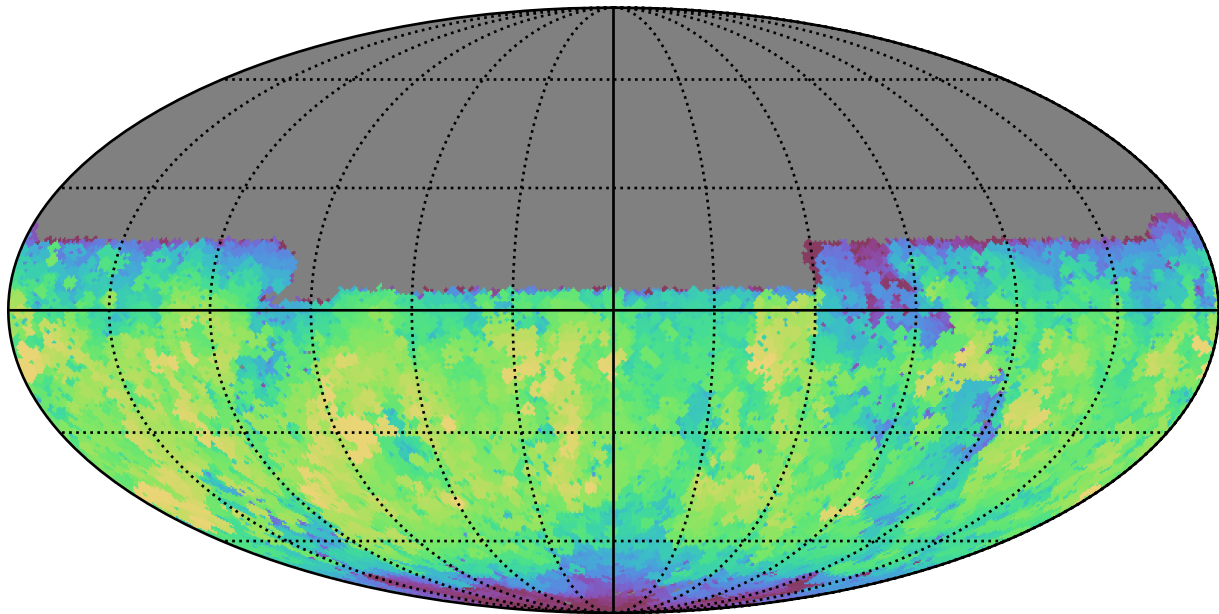
baseline_v3.5_10yrs Yr 1 y band: Max fiveSigmaDepth
