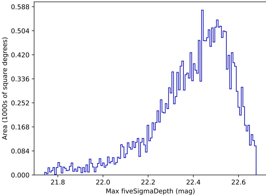
baseline_v3.5_10yrs Yr 1 y band: Max fiveSigmaDepth
