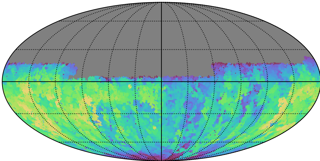
baseline_v3.5_10yrs Yr 1 u band: Max fiveSigmaDepth
