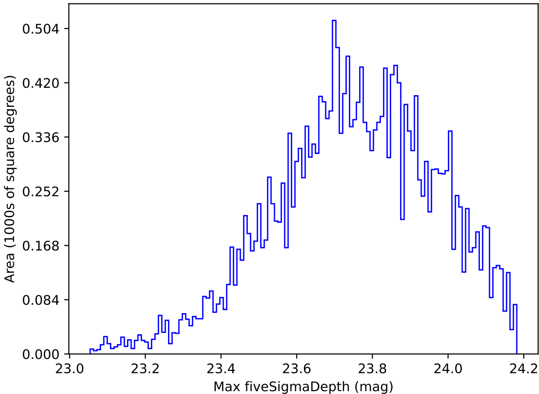
baseline_v3.5_10yrs Yr 1 u band: Max fiveSigmaDepth
