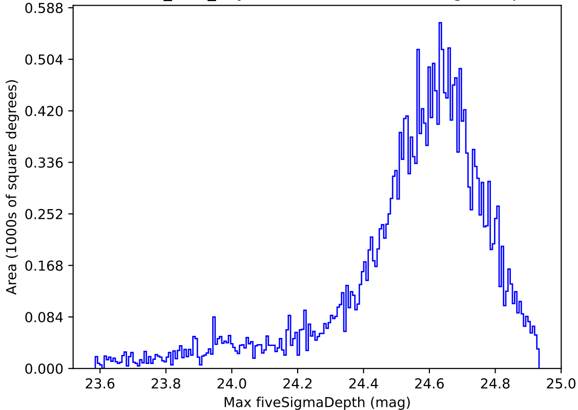
baseline_v3.5_10yrs Yr 1 r band: Max fiveSigmaDepth
