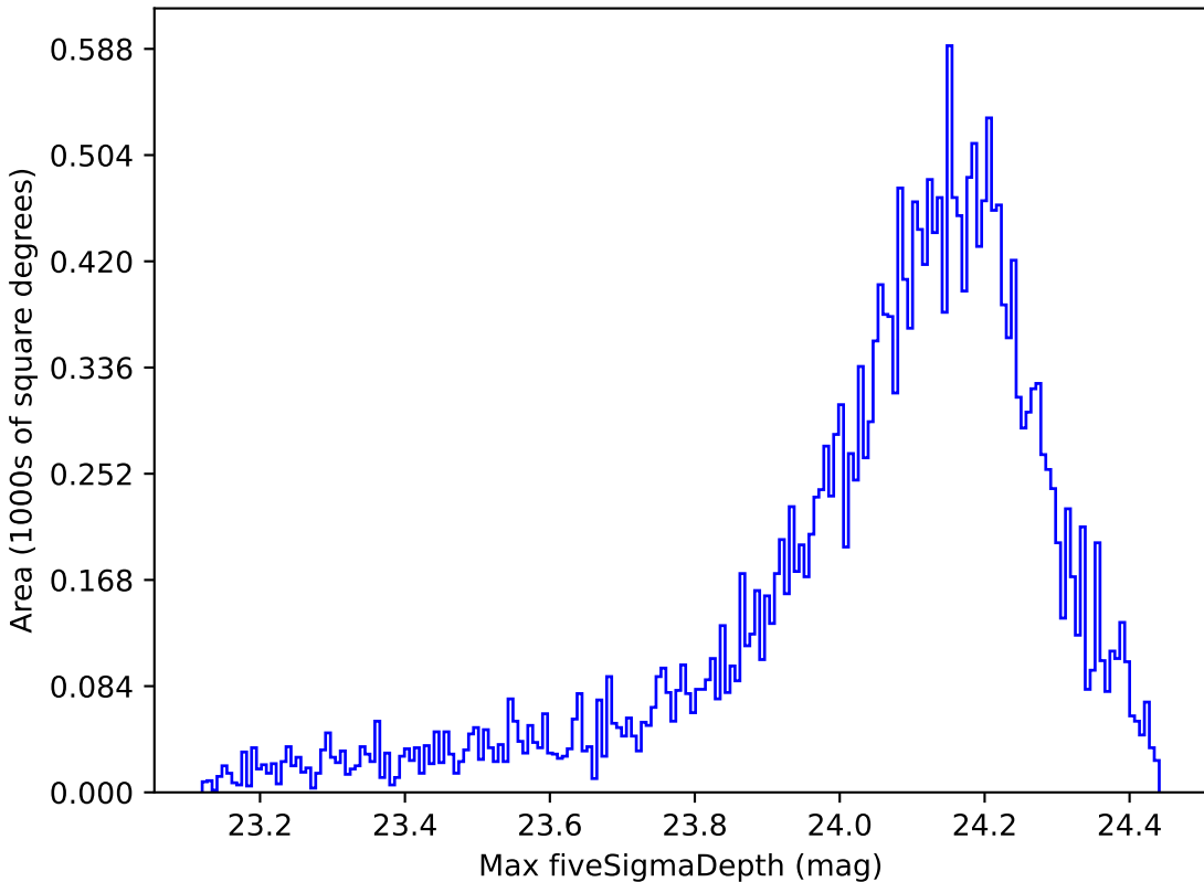
baseline_v3.5_10yrs Yr 1 i band: Max fiveSigmaDepth
