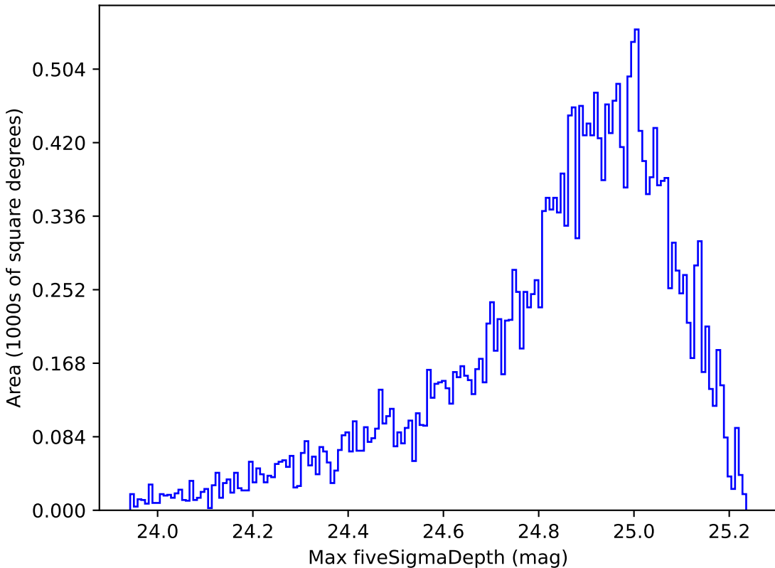
baseline_v3.5_10yrs Yr 1 g band: Max fiveSigmaDepth
