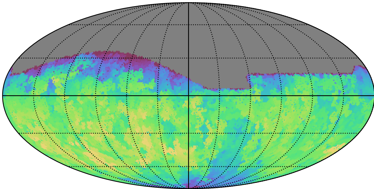
baseline_v3.5_10yrs Yr 1 all bands: Max fiveSigmaDepth
