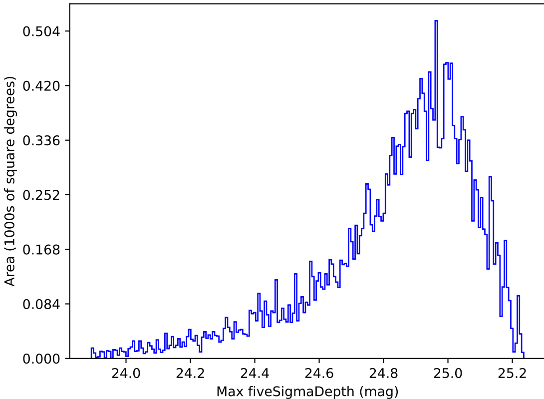
baseline_v3.5_10yrs Yr 1 all bands: Max fiveSigmaDepth
