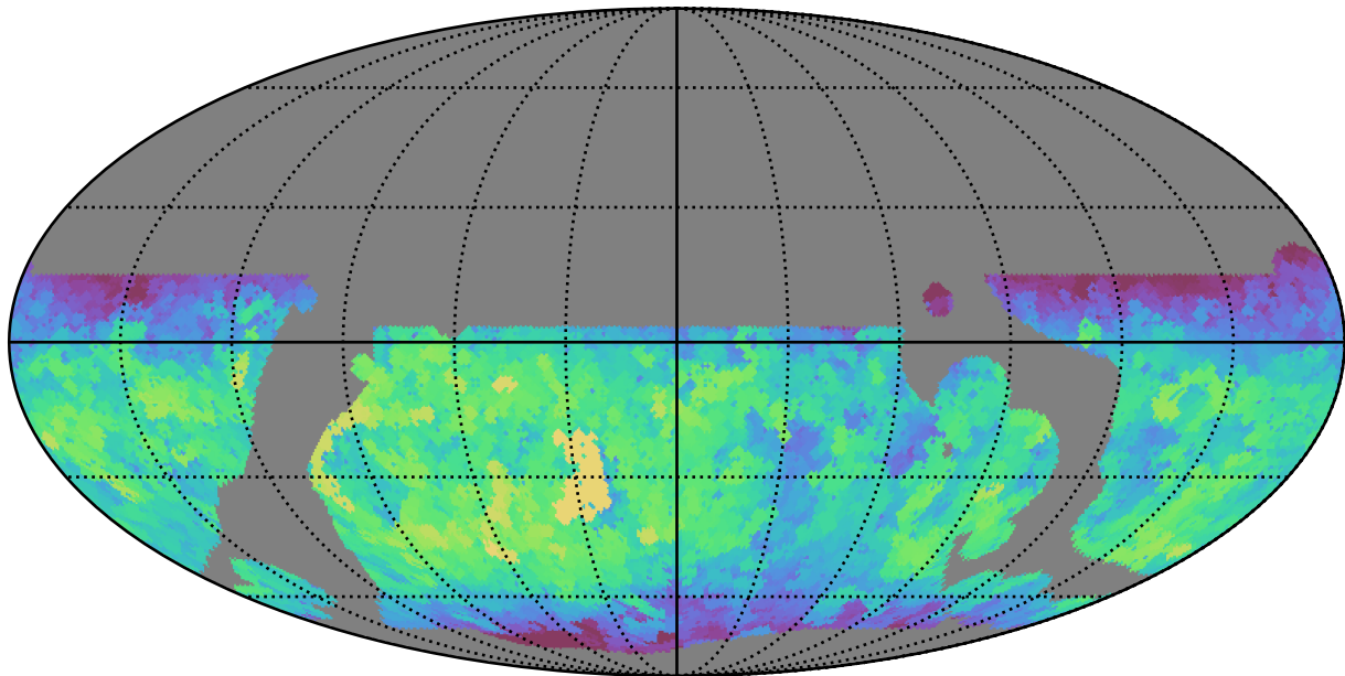
baseline_v3.5_10yrs WFD z band: Max fiveSigmaDepth
