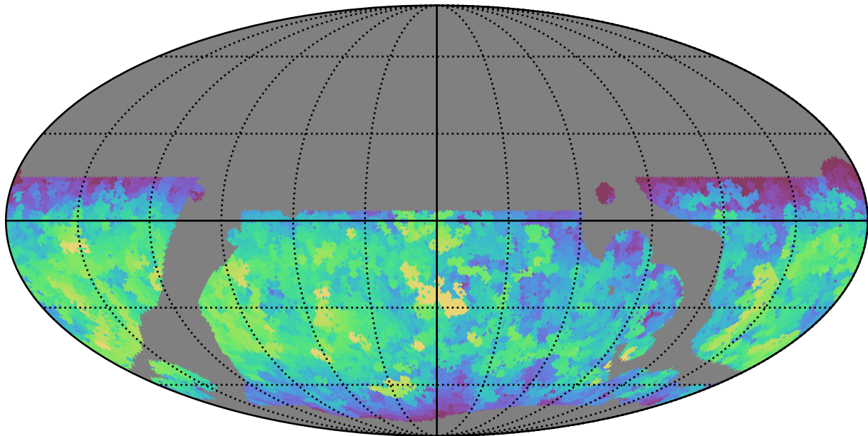
baseline_v3.5_10yrs WFD u band: Max fiveSigmaDepth
