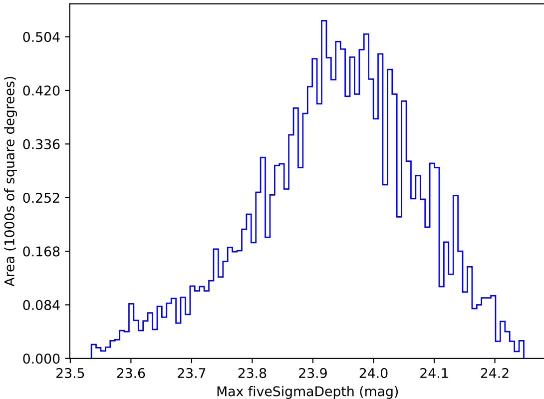
baseline_v3.5_10yrs WFD u band: Max fiveSigmaDepth
