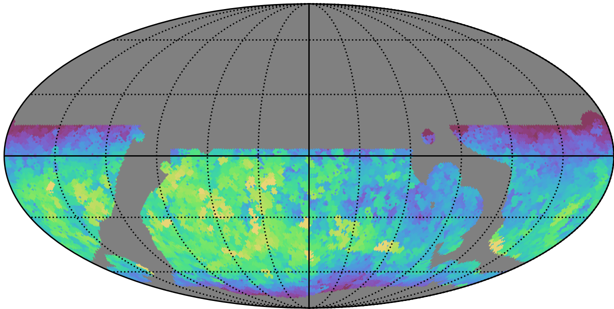
baseline_v3.5_10yrs WFD r band: Max fiveSigmaDepth
