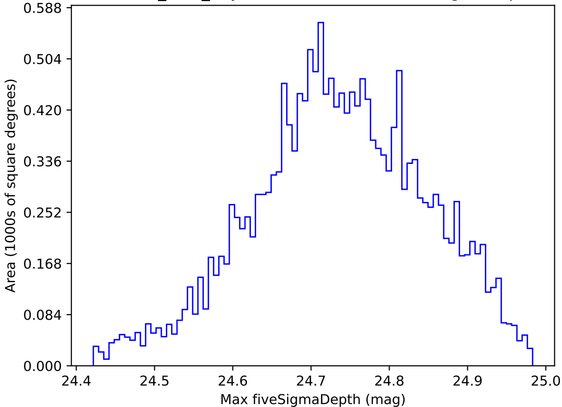
baseline_v3.5_10yrs WFD r band: Max fiveSigmaDepth
