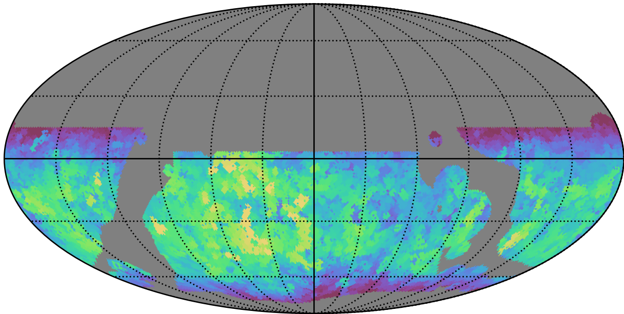
baseline_v3.5_10yrs WFD i band: Max fiveSigmaDepth
