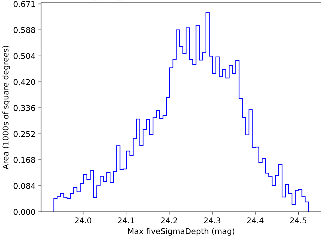
baseline_v3.5_10yrs WFD i band: Max fiveSigmaDepth
