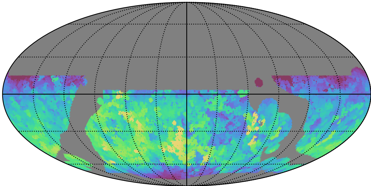
baseline_v3.5_10yrs WFD g band: Max fiveSigmaDepth
