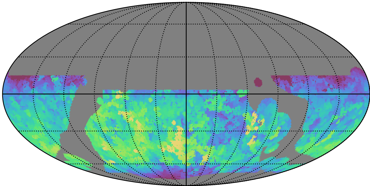
baseline_v3.5_10yrs WFD all bands: Max fiveSigmaDepth
