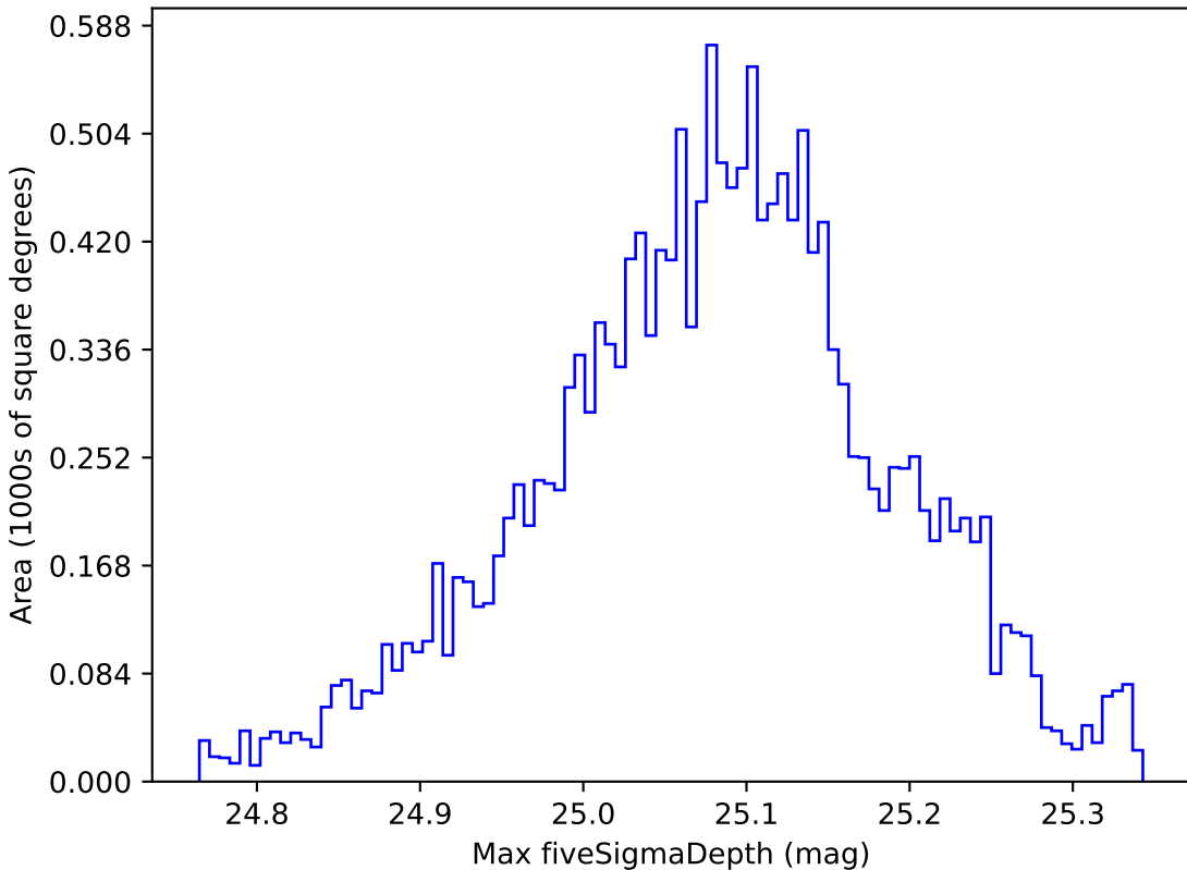
baseline_v3.5_10yrs WFD all bands: Max fiveSigmaDepth
