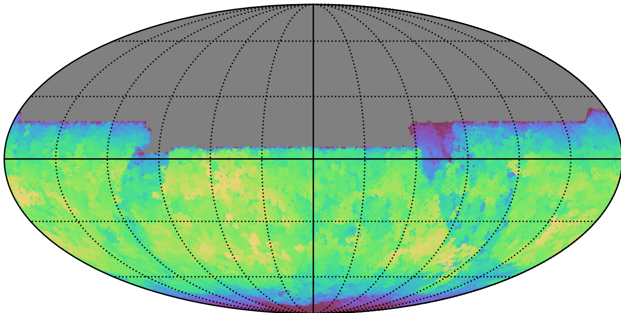
baseline_v3.5_10yrs All sky y band: Max fiveSigmaDepth
