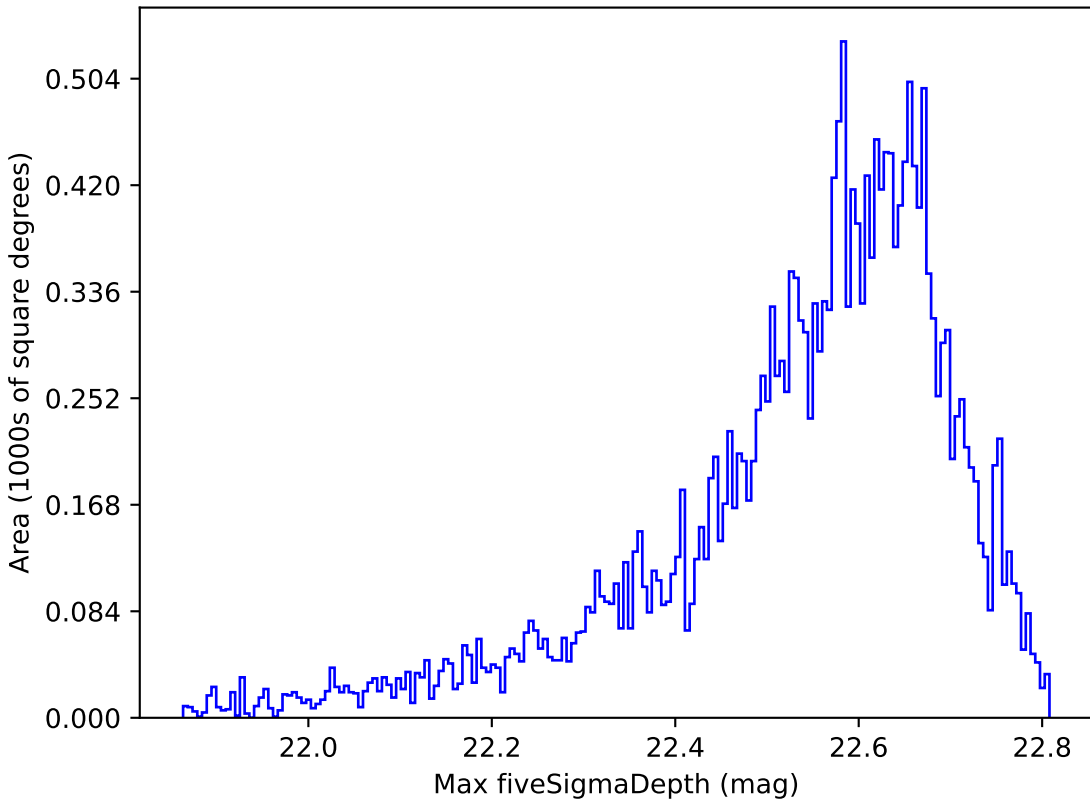
baseline_v3.5_10yrs All sky y band: Max fiveSigmaDepth
