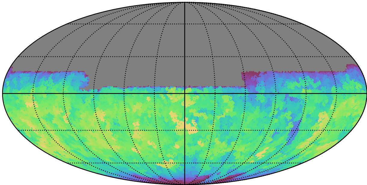
baseline_v3.5_10yrs All sky u band: Max fiveSigmaDepth
