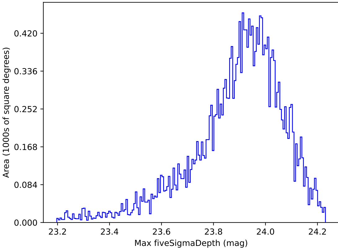
baseline_v3.5_10yrs All sky u band: Max fiveSigmaDepth
