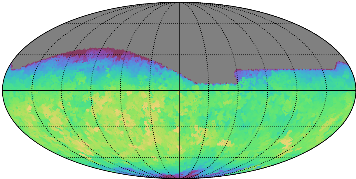
baseline_v3.5_10yrs All sky r band: Max fiveSigmaDepth
