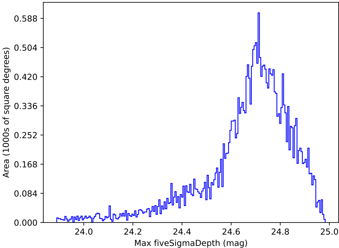
baseline_v3.5_10yrs All sky r band: Max fiveSigmaDepth
