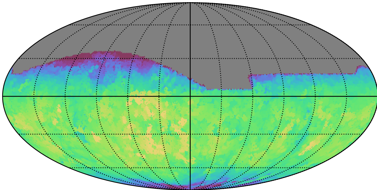
baseline_v3.5_10yrs All sky i band: Max fiveSigmaDepth
