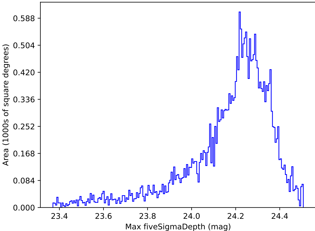
baseline_v3.5_10yrs All sky i band: Max fiveSigmaDepth
