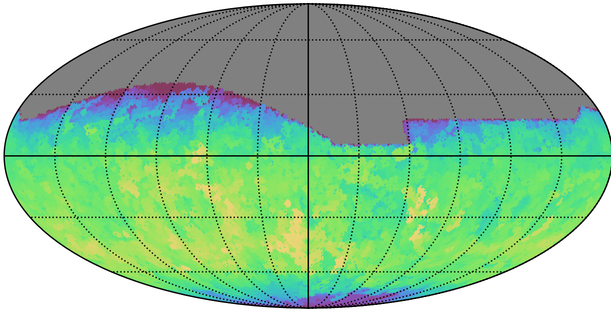
baseline_v3.5_10yrs All sky g band: Max fiveSigmaDepth
