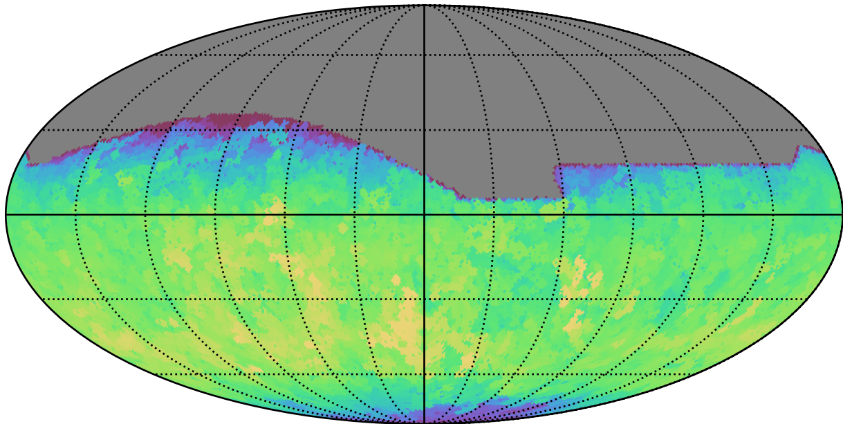
baseline_v3.5_10yrs All sky all bands: Max fiveSigmaDepth
