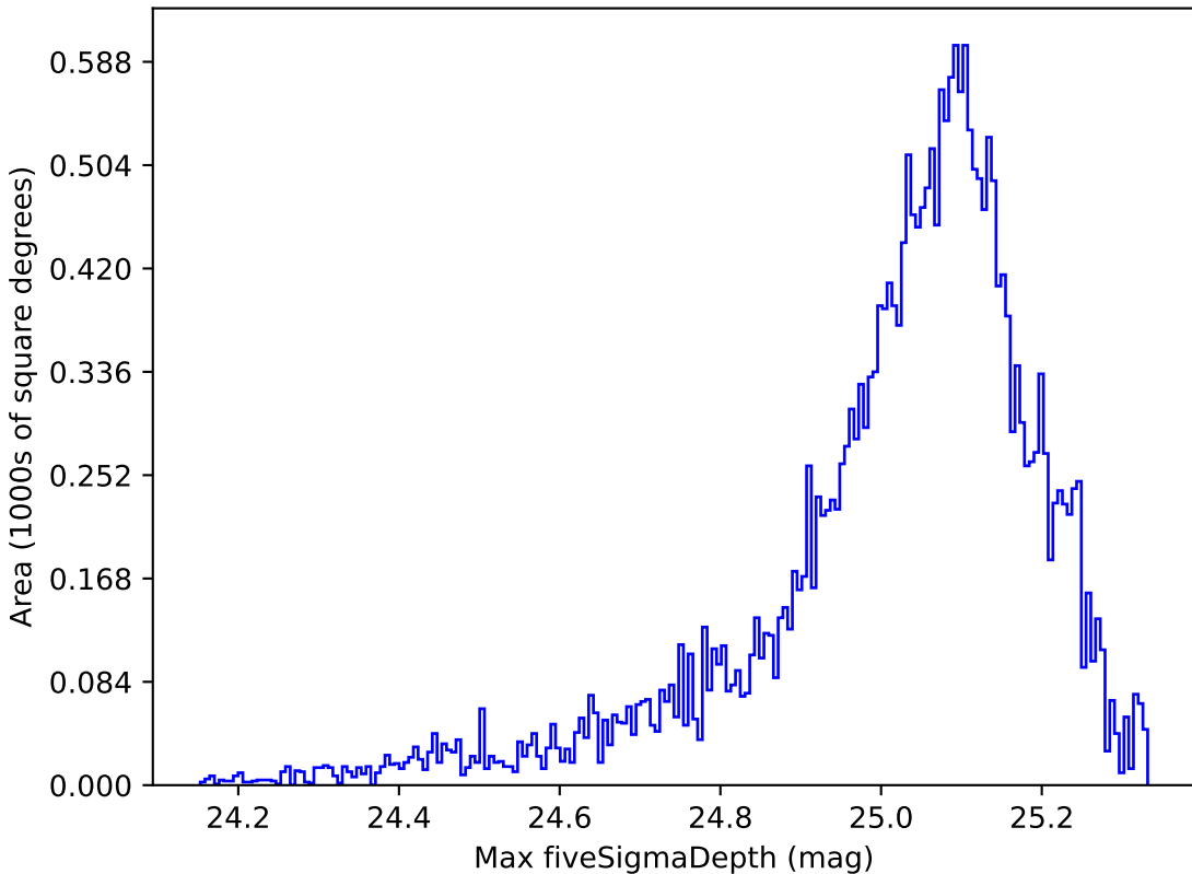
baseline_v3.5_10yrs All sky all bands: Max fiveSigmaDepth
