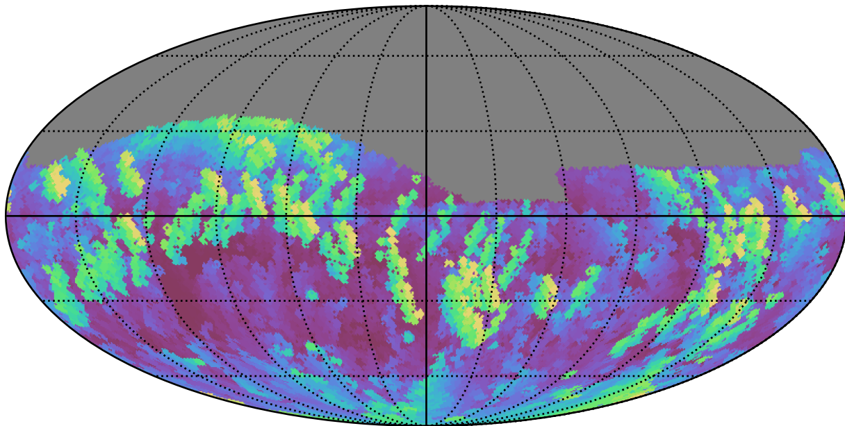
baseline_v3.5_10yrs Yr 1 z band: Max airmass
