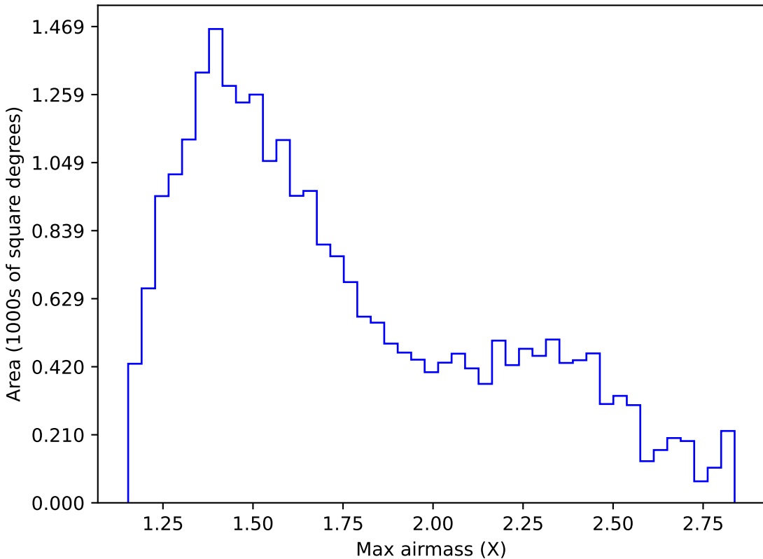
baseline_v3.5_10yrs Yr 1 z band: Max airmass
