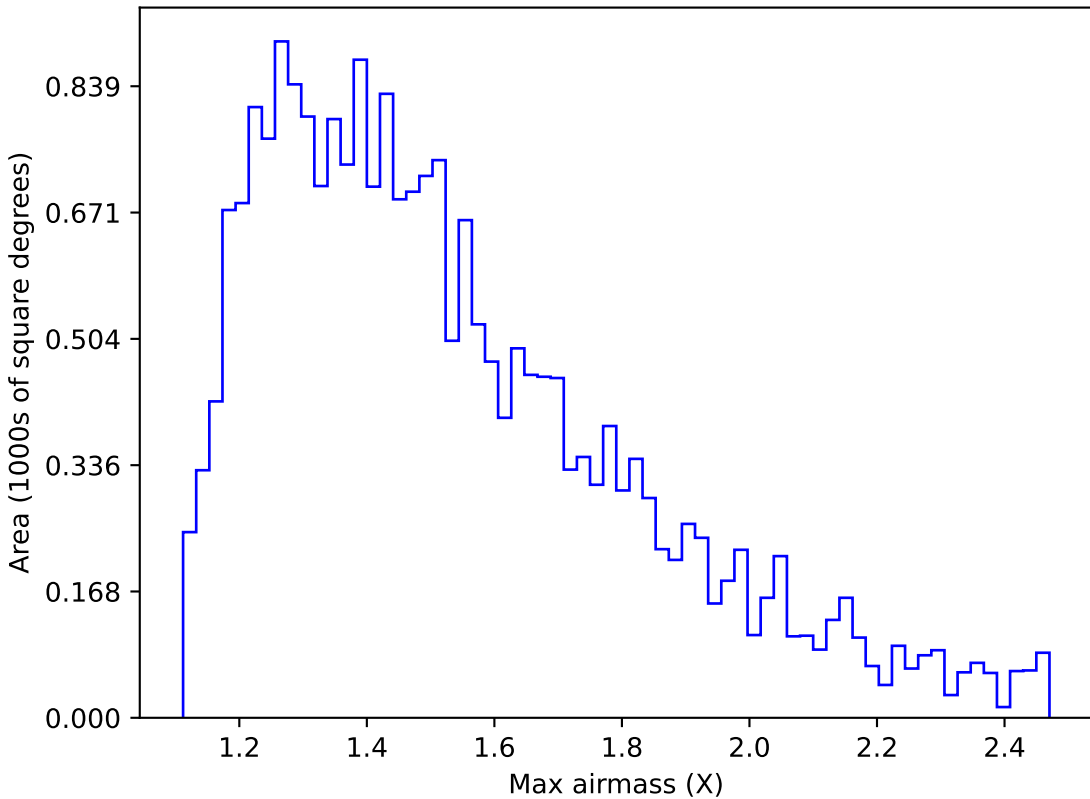
baseline_v3.5_10yrs Yr 1 u band: Max airmass
