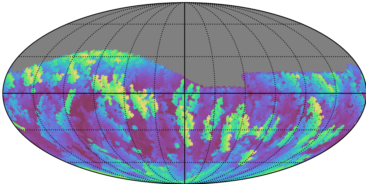
baseline_v3.5_10yrs Yr 1 r band: Max airmass
