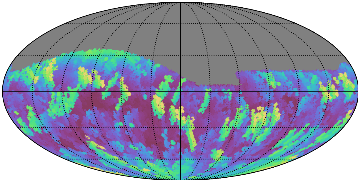
baseline_v3.5_10yrs Yr 1 i band: Max airmass
