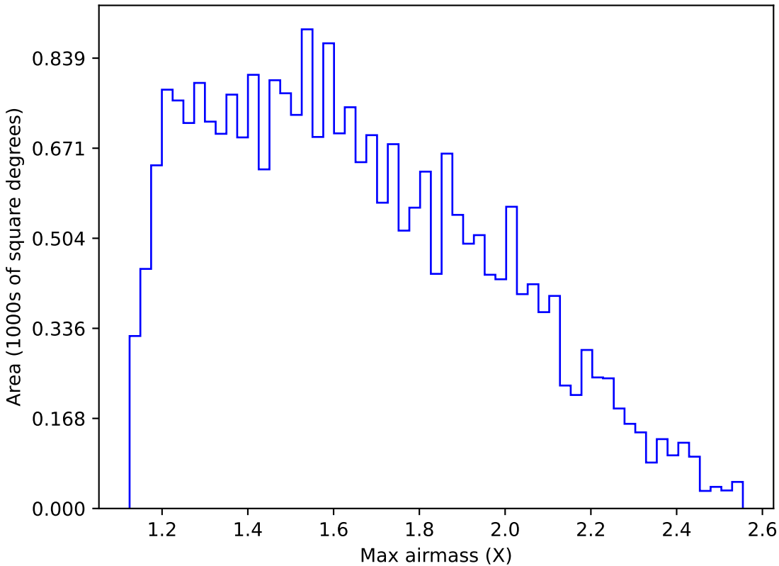
baseline_v3.5_10yrs Yr 1 g band: Max airmass
