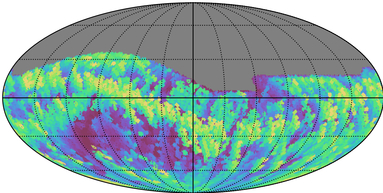
baseline_v3.5_10yrs Yr 1 all bands: Max airmass
