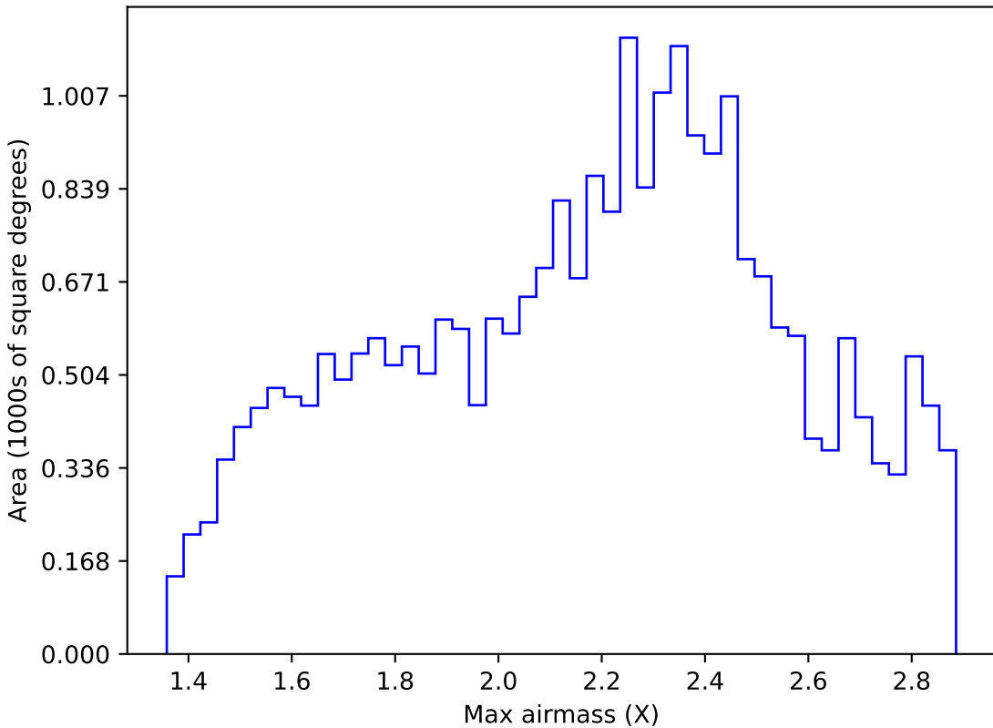
baseline_v3.5_10yrs Yr 1 all bands: Max airmass
