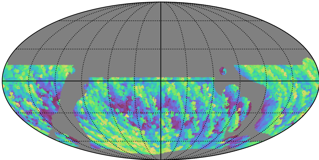
baseline_v3.5_10yrs WFD y band: Max airmass
