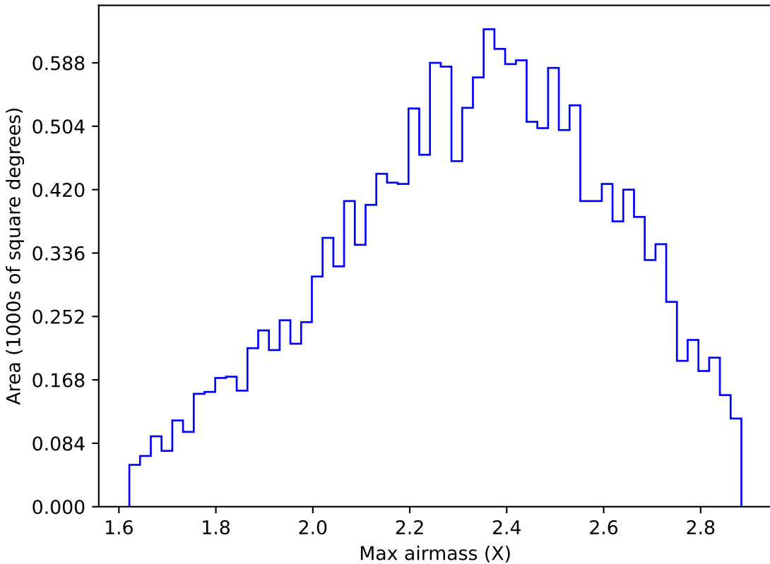
baseline_v3.5_10yrs WFD y band: Max airmass
