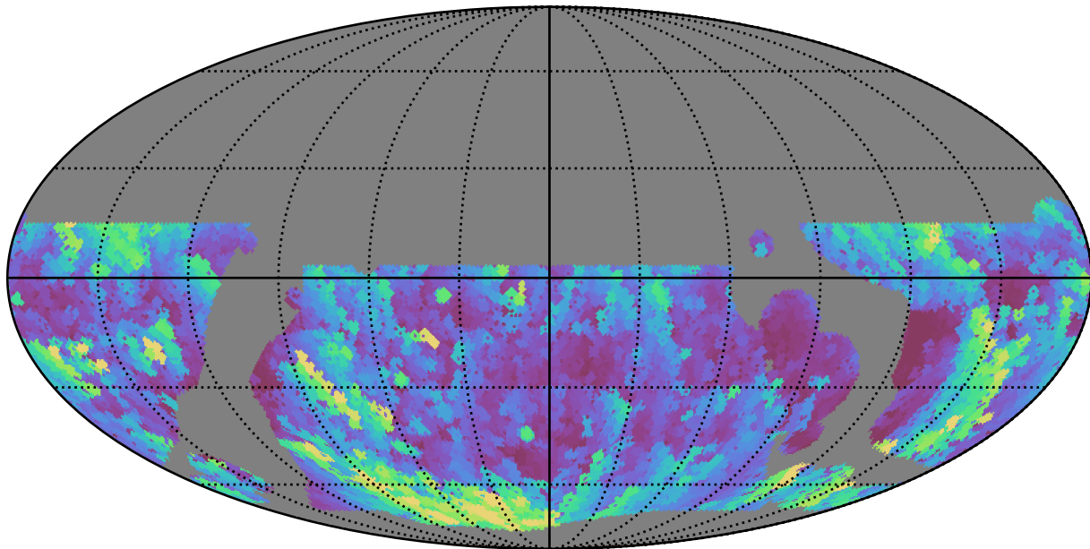
baseline_v3.5_10yrs WFD u band: Max airmass
