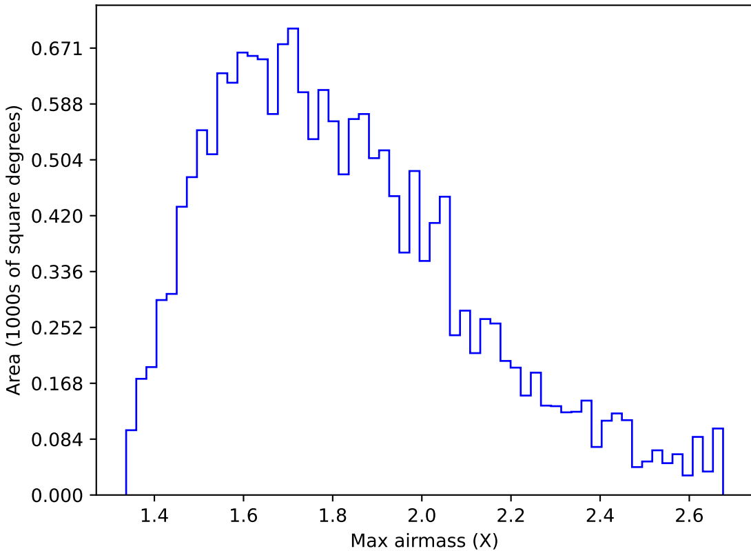
baseline_v3.5_10yrs WFD u band: Max airmass
