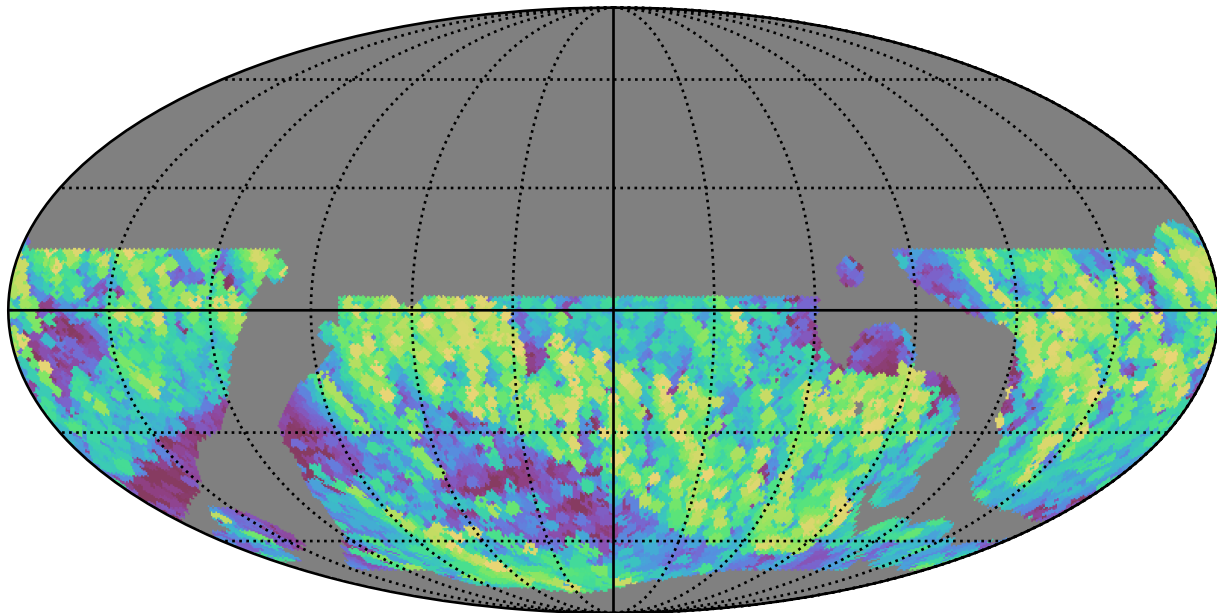
baseline_v3.5_10yrs WFD r band: Max airmass
