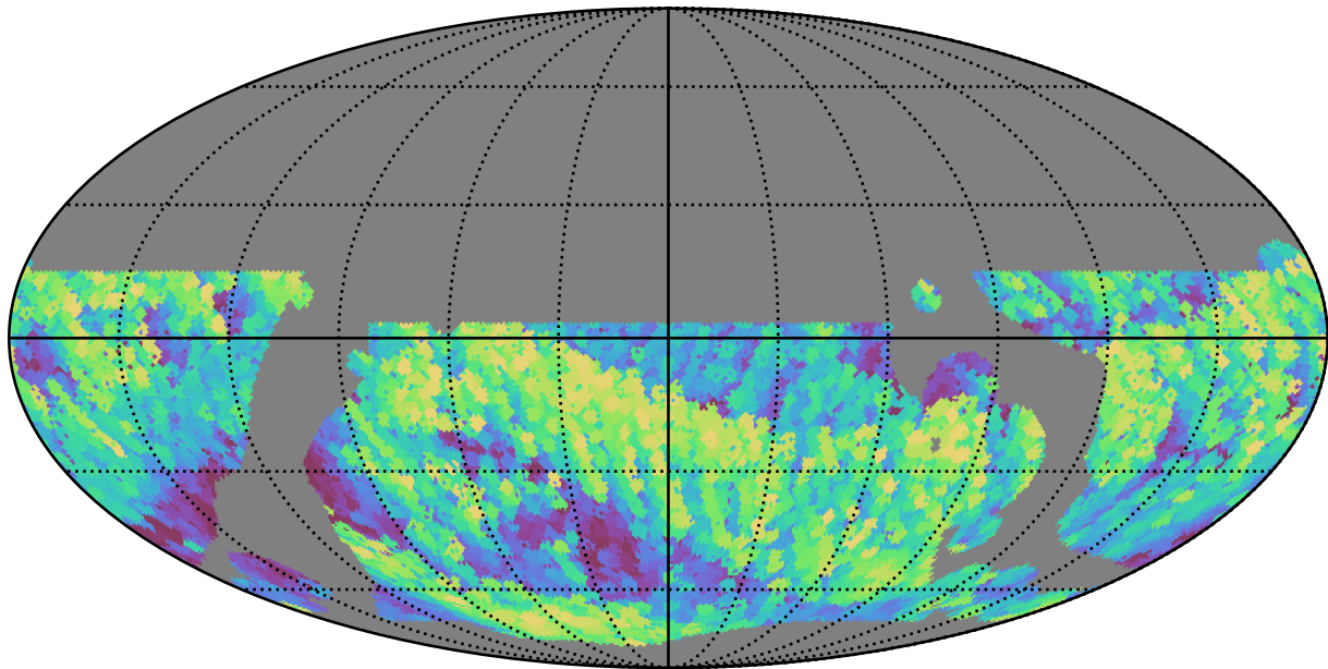
baseline_v3.5_10yrs WFD i band: Max airmass
