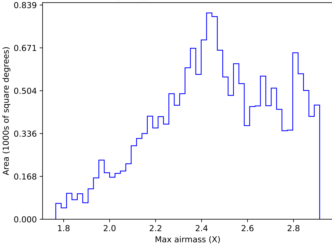
baseline_v3.5_10yrs WFD i band: Max airmass
