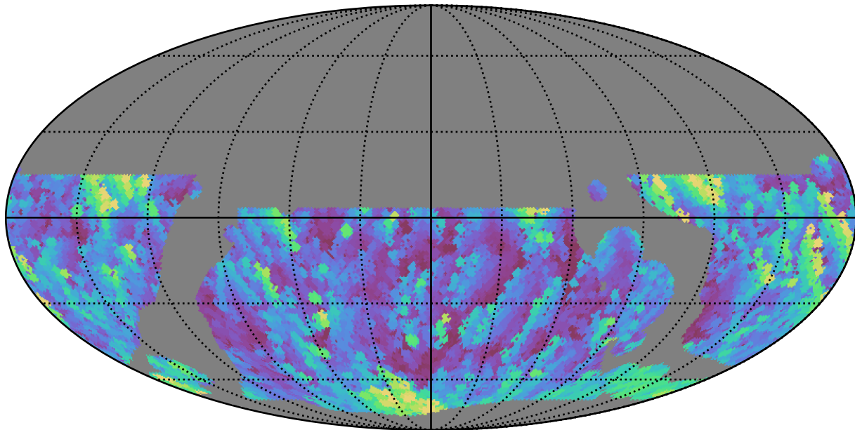
baseline_v3.5_10yrs WFD g band: Max airmass
