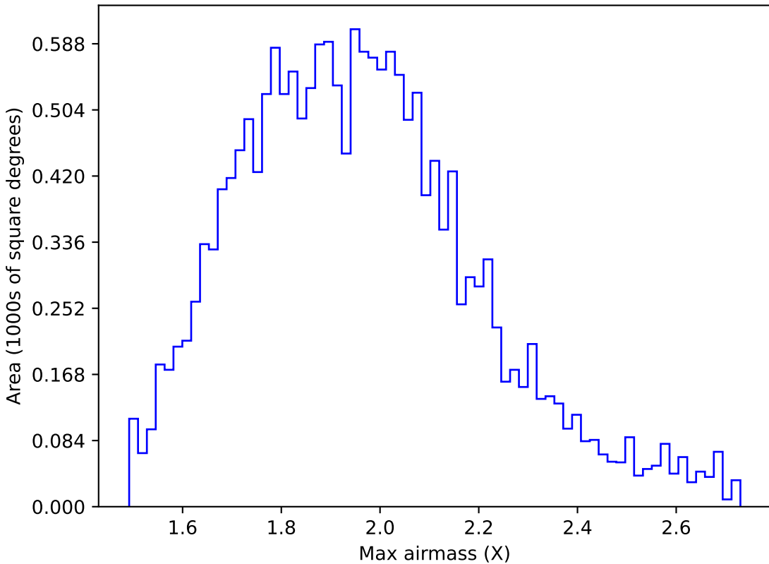
baseline_v3.5_10yrs WFD g band: Max airmass
