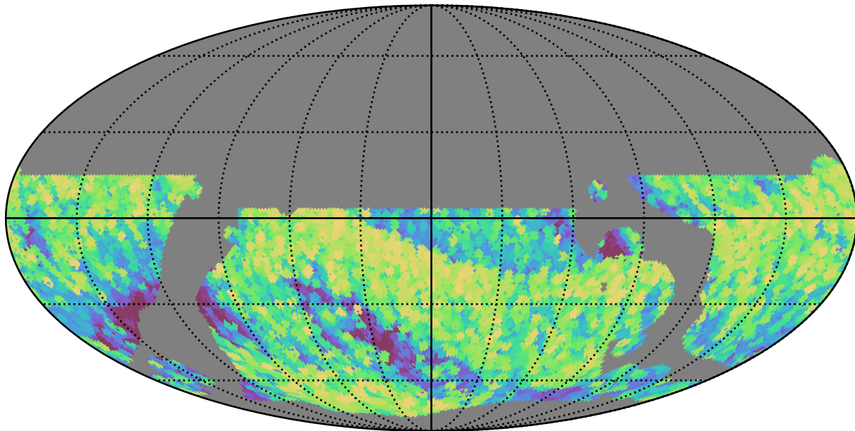
baseline_v3.5_10yrs WFD all bands: Max airmass
