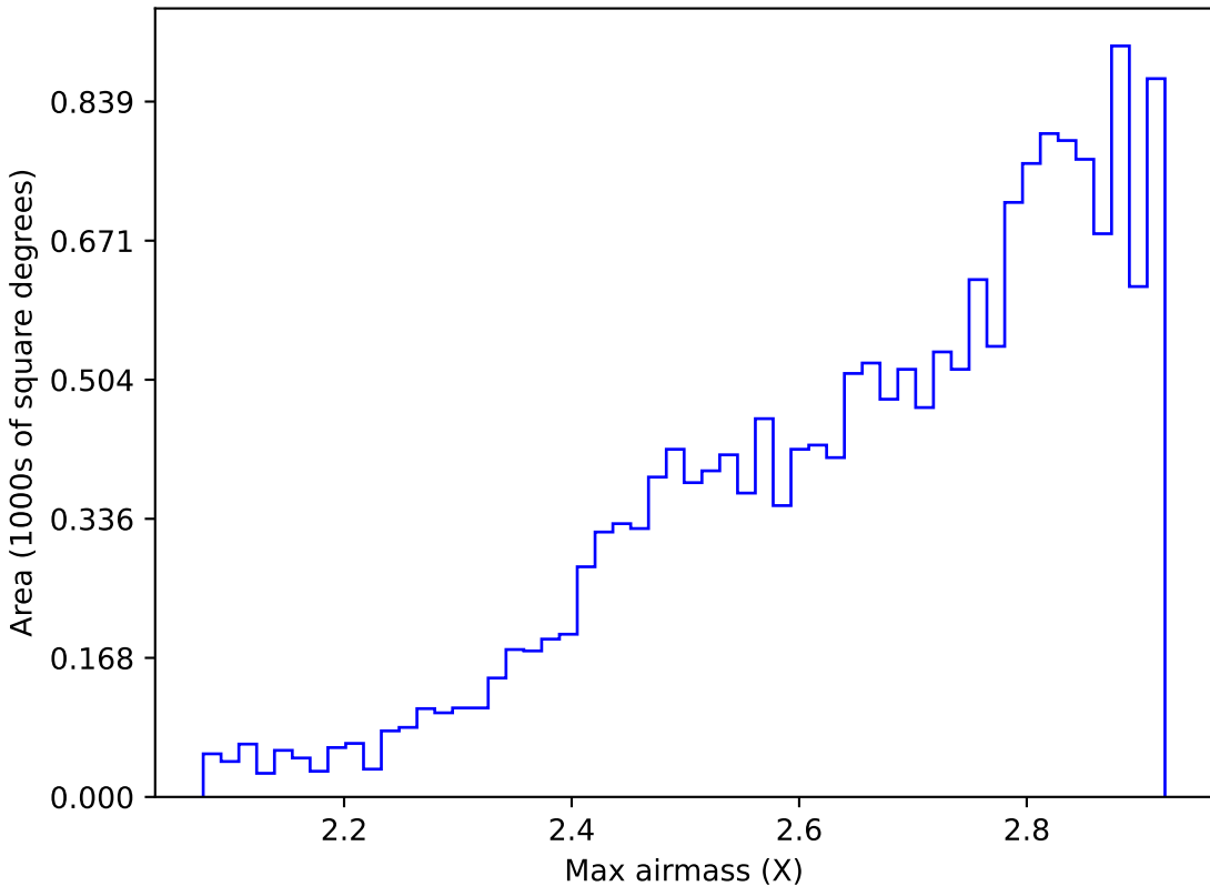
baseline_v3.5_10yrs WFD all bands: Max airmass
